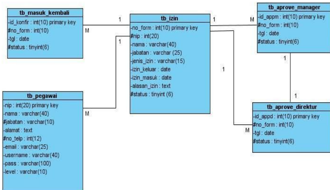
Figure 3. Calss Diagram
